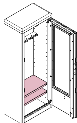
FIXED, METAL SHELVES
