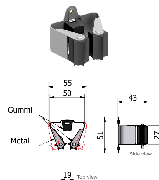
PRAX gun holder
